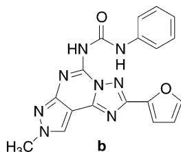
Chart 1. Structure of the pyrazolo-triazolo-pyrimidines a and b as hA 3 adenosine receptor antagonists.
