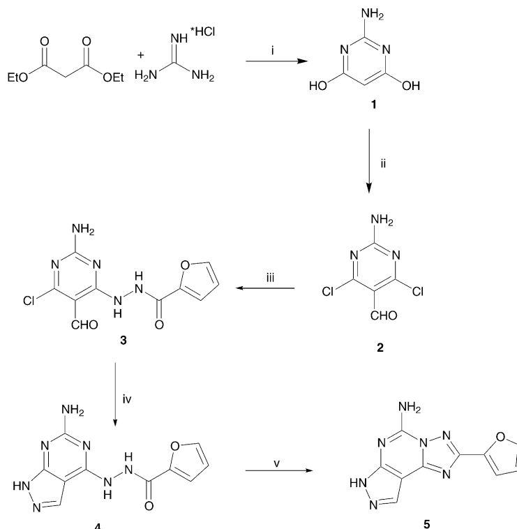
Scheme 1. Reagents: (i) EtONa, EtOH abs; (ii) POCl 3 , DMF, Rfx; (iii) 2-furoic acid hydrazide, THF; (iv) hydrazine·H 2 O, 2-methoxyethanol; (v) HMDS, BSA, DMF.
