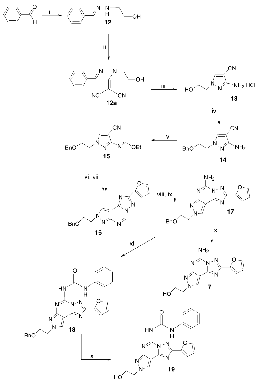
Scheme 4. Reagents: (i) 2-hydroxyethylhydrazine, abs EtOH; (ii) ethoxymethylene-malono nitrile, benzene; (iii) concd HCl; (iv) benzylbromide, 60% NaH; (v) \text{HC(OEt)}_3 , rfx; (vi) 2-furoic acid hydrazide, 2-methoxyethanol; (vii) \text{Ph}_2\text{O} , 260 °C; (viii) aq HCl 10%; (ix) \text{NH}_2\text{CN} , pTsOH; (x) \text{HCO}_2\text{NH}_4 , Pd/C 10%; (xi) phenylisocyanate, TEA.
