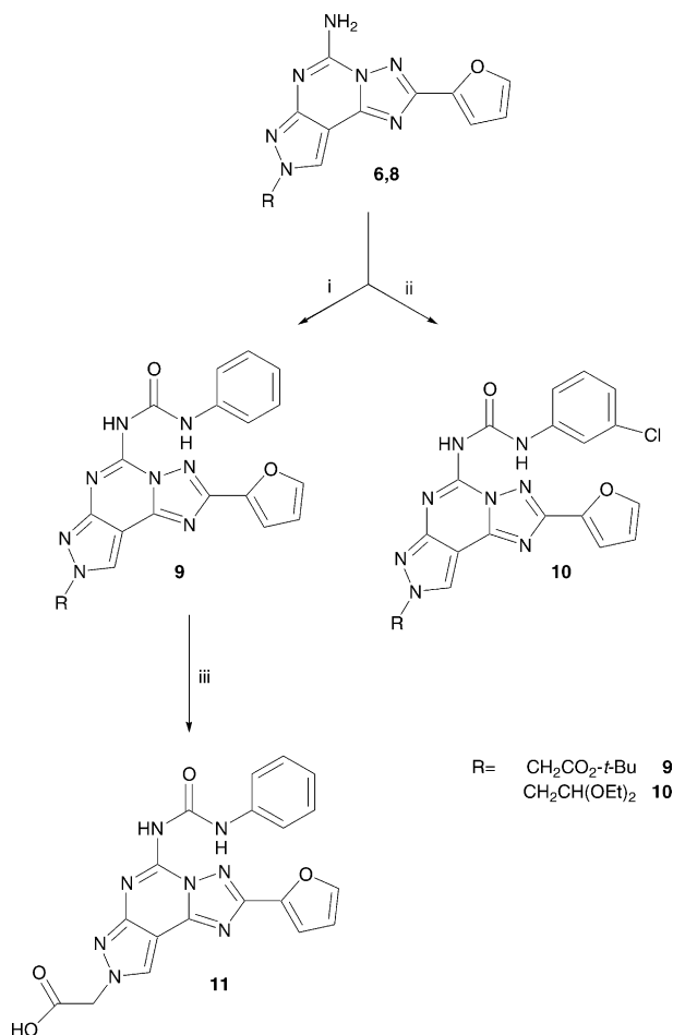
Scheme 3. Reagents: (i) phenylisocyanate, TEA, dry \text{CH}_3\text{CN} ; (ii) 3-chlorophenylisocyanate, TEA, dry \text{CH}_3\text{CN} ; (iii) TFA, rt.
